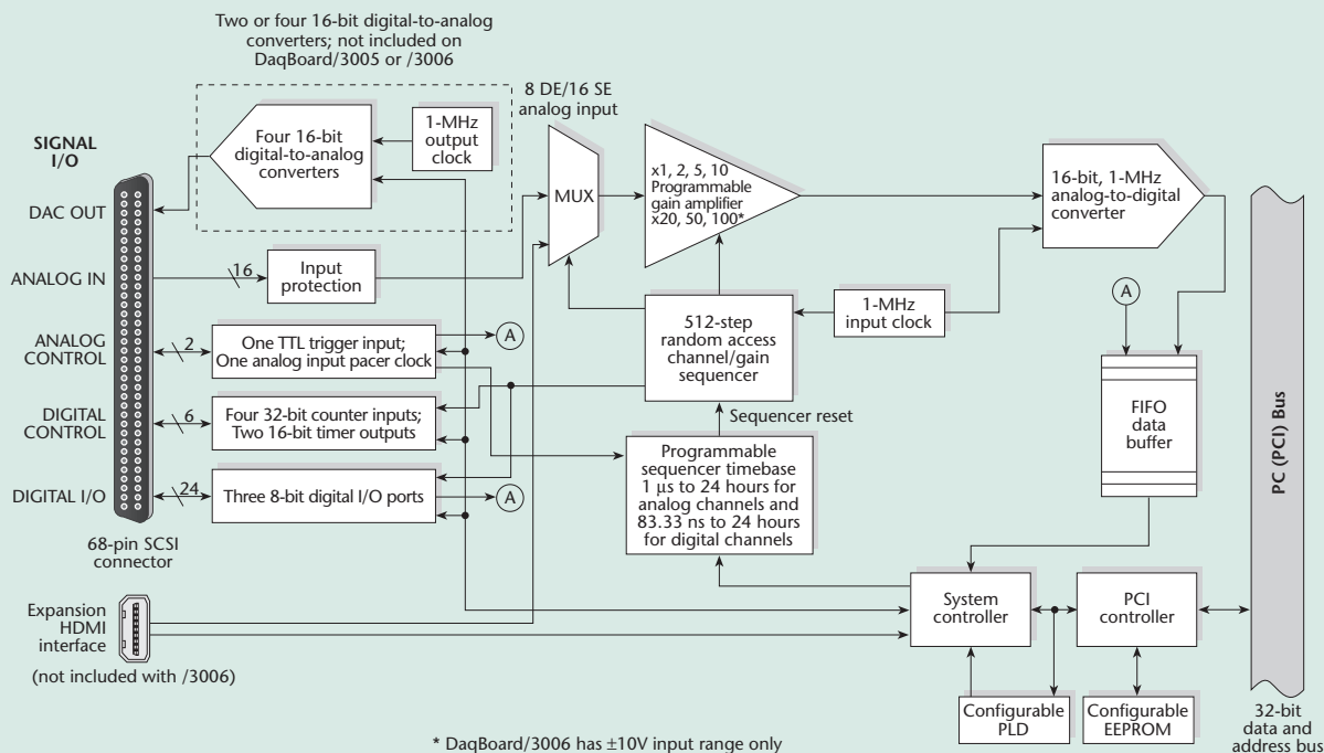
DaqBoard/3000 Series Block Diagram
